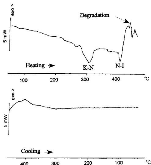
Figure 5 DSC heat-cool cycle of the AD copolyester: (a) the K-N and the N-I transitions are both observed in the first heating scan; (b) on the cooling scan after isotropization, the reverse transitions are affected by the degradation that had occurred on heating.
