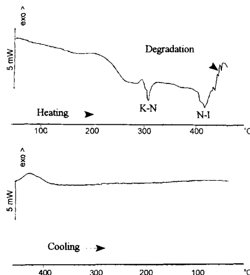
Figure 4 DSC heat-cool cycle of the ND copolyester: (a) the heating scan shows two major peaks, corresponding to the K - N and N - I transitions; (b) on the cooling scan after isotropization, the reverse transitions are affected by the degradation that had occurred on heating.
