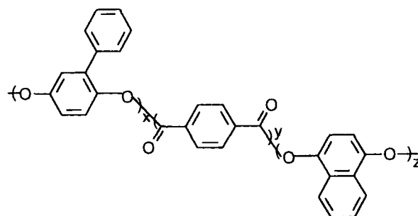
Scheme 3 Polymer A is the copolyester of TA, PHQ, and 1,4-ND.
