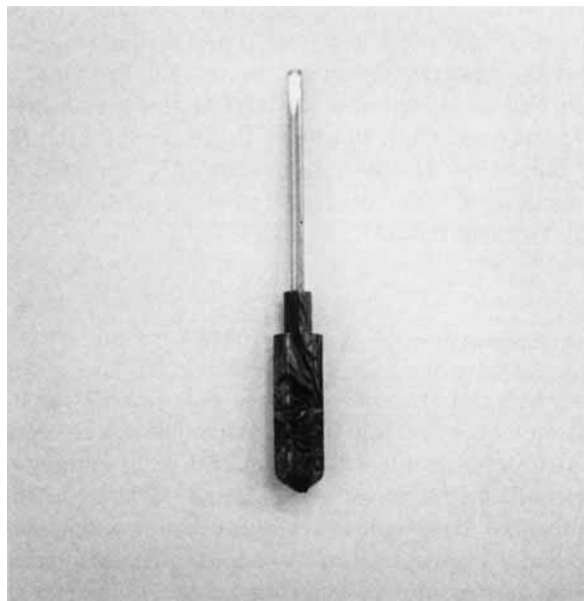
Figure 1 Injection-molded screw driver handle, formed from the ND polyester. Note the weld lines caused by jetting. This occurs typically with LCPs when using molds with gating designed for conventional thermoplastics.
