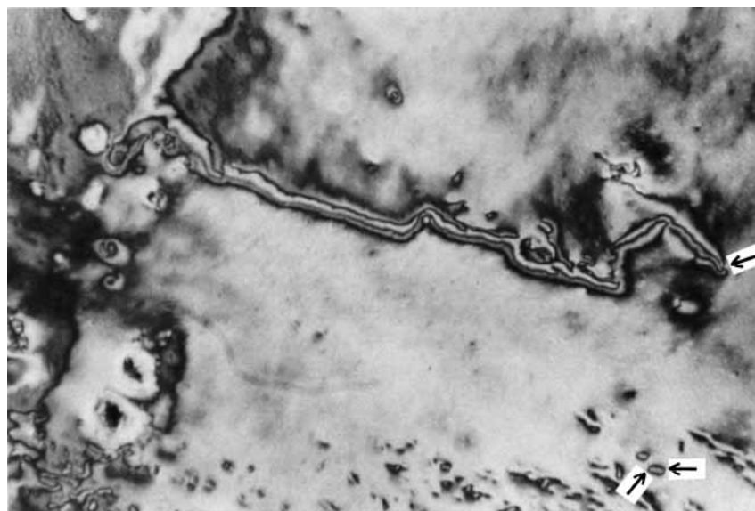
Figure 2 Nematic texture of the LCP of the ND copolyester. Crossed polars, 385°C. The orientation of the polars is north-south and east-west. The double arrows (bottom) show singularities with s = \pm\frac{1}{2} . Single arrow (right edge) shows singularity with s = 1 .
