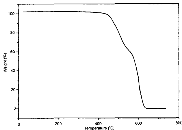
Figure 8 Thermogravimetric analysis curve of the ND copolyester.
