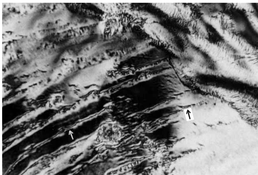
Figure 3 Nematic texture of the AD copolyester. Black arrow on the right side shows an inversion wall, starting and ending at singularities with s = \pm\frac{1}{2} . White arrow on the left side shows another inversion wall, whose center appears as a black line bordered by two bright stripes. Crossed polars, 385°C. The orientation of the polars is north–south and east–west.
